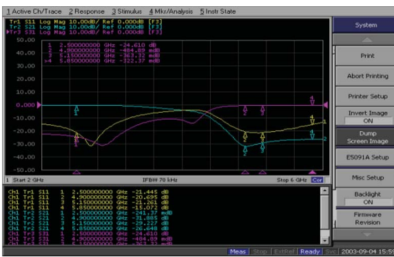
RFDIP2012100L4T
