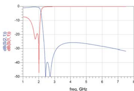
RFLPF1005040A1T
