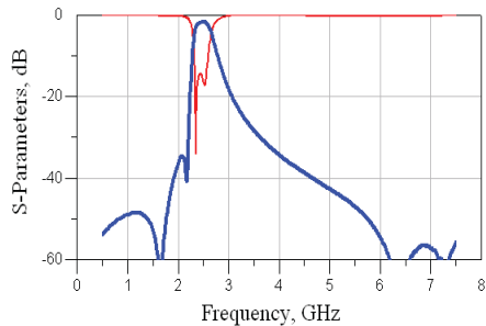
RFBPF2520100A6T
