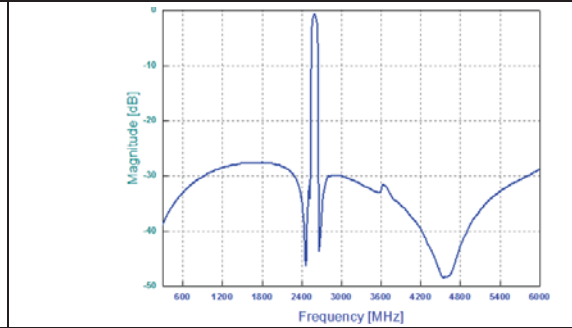
SF14112350B4001T
