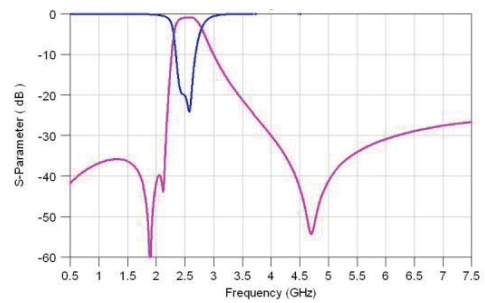
RFBPF2012040AHT
