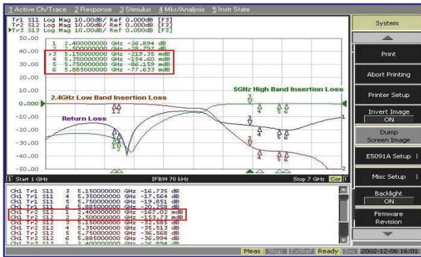
RFDIP2012100L0T
